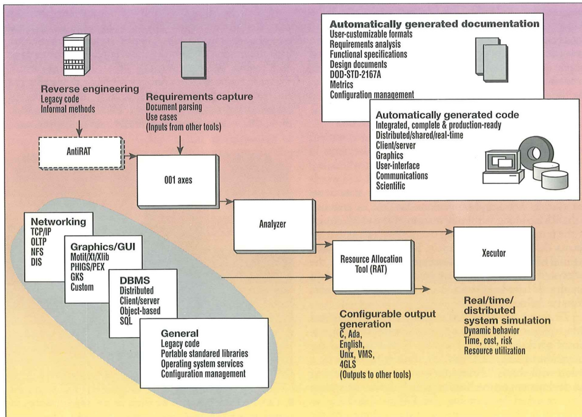
Figure 9. A seamless, open architecture environment, the 001 tool suite inherently supports an integration of function- and object-oriented development.
