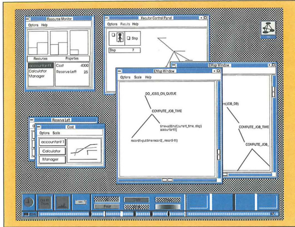
Figure 7. The Xecutor runs the FMaps and TMaps in the form of EMaps (instantiations of FMaps) and OMaps (instantiations of TMaps). With the Xecutor simulator, the behavior and performance of a system can be analyzed.
