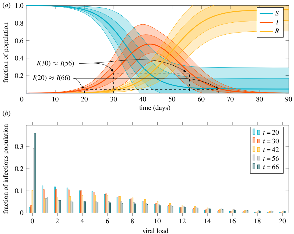
Figure 5. Epidemic curve and viral load distributions for a rising, stationary and falling epidemic. (a) Epidemic curve showing the susceptible ( S ), infectious ( I ) and removed ( R ) observables for a population of 10 000 individuals calibrated for a reproduction number of 3. Envelopes show 1 and 2 s.d. over 128 simulations. Marked on the graph are two pairs of time points where the mean number of infectious individuals are equal as the epidemic rises and falls. (b) Viral load distribution at different points of the epidemic trajectory showing a rising t \in \{20, 30\} , stationary t = 42 and falling t \in \{56, 66\} epidemic. Viral load in arbitrary logarithmic units. The probability masses of distributions are shifted to the left (lower viral loads) for a rising epidemic and the distribution for a falling epidemic is in fact bimodal with most infected individuals on the point of recovery but a significant number with slowly decaying high viral loads. (Online version in colour.)
